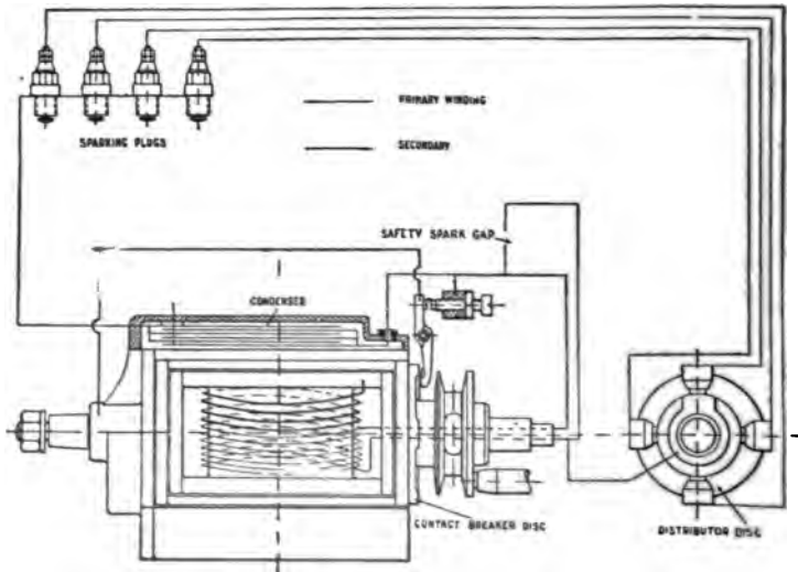
FIG. 198.—Circuit Diagram showing the Simms-Bosch High-tension Magneto wired up to spark a four-cylinder engine.
